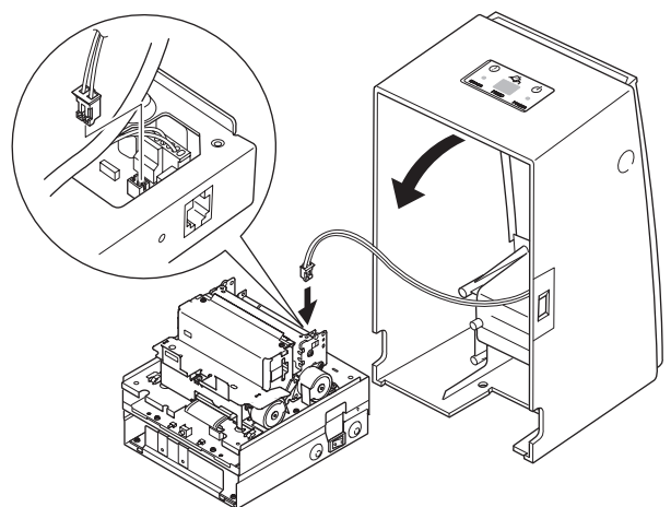
Fig.7 Connecting Connector Cable
