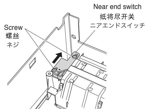
Fig.4 Positioning the Near End Switch
