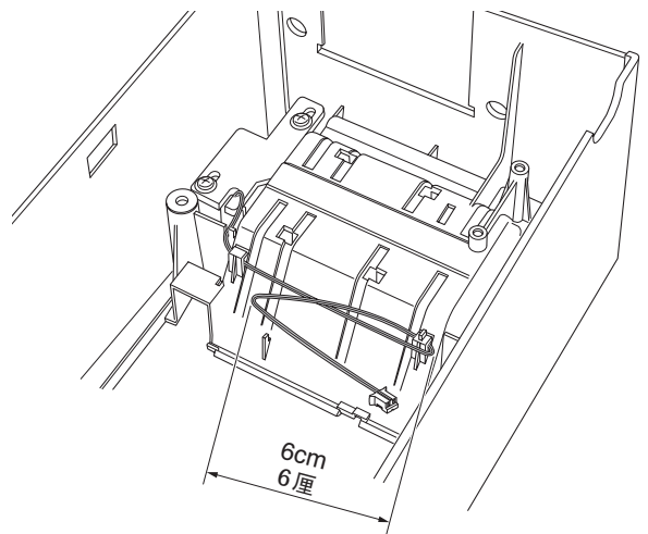
Fig.6 Bundling the Connector Cable
