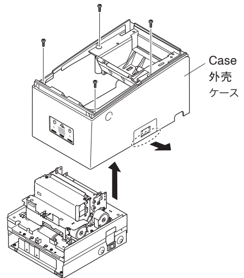
Fig.2 Removing the Case
