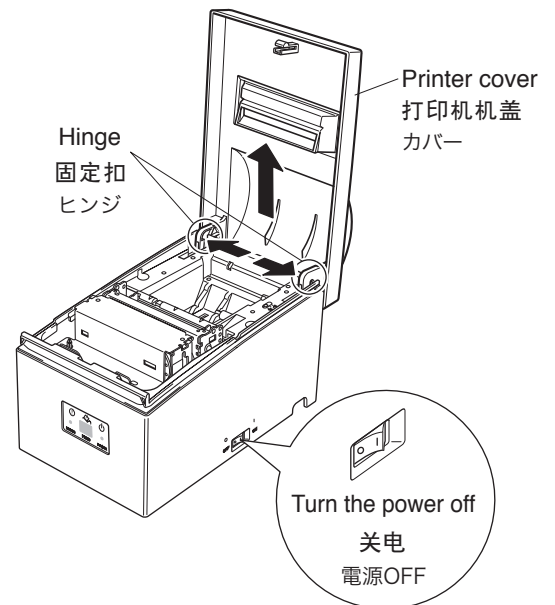
Fig.1 Removing the Printer Cover
